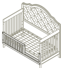
Toddler Rail – 1515 W:57.5 x D:31.5 x H:50
